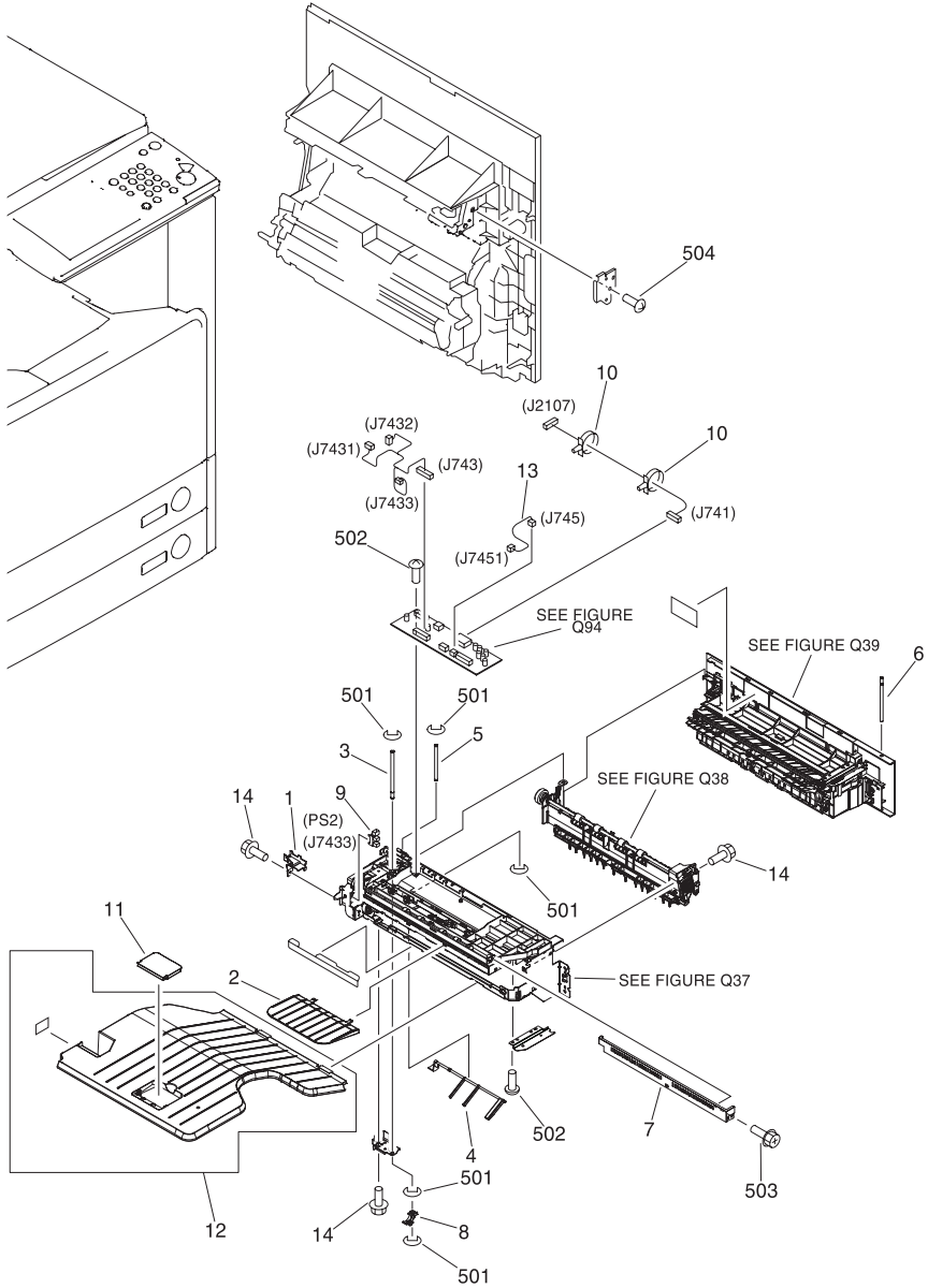
FIGURE Q11 INTERNAL DELIVERY MAIN BODY
