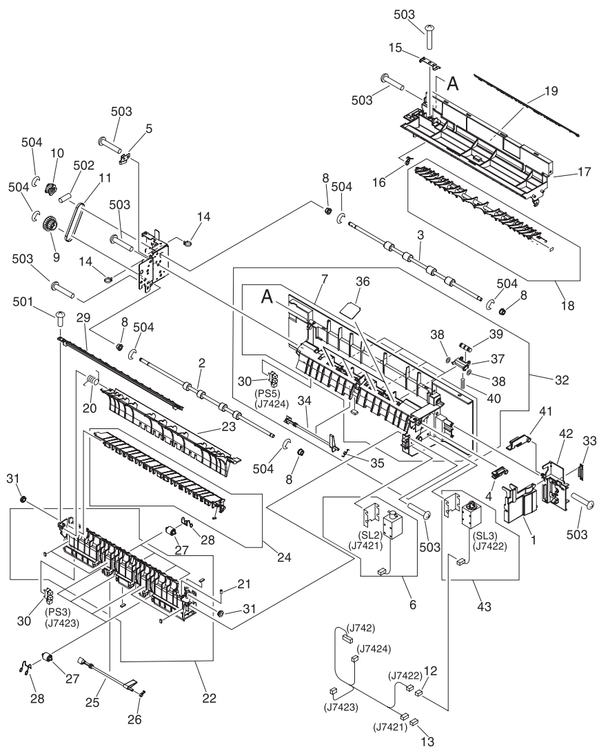
FIGURE Q39 3RD DELIVERY FRAME ASSEMBLY
