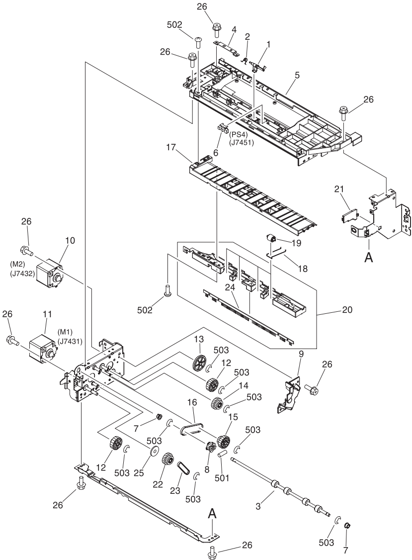
FIGURE Q37 2ND UPPER DELIVERY ASSEMBLY
